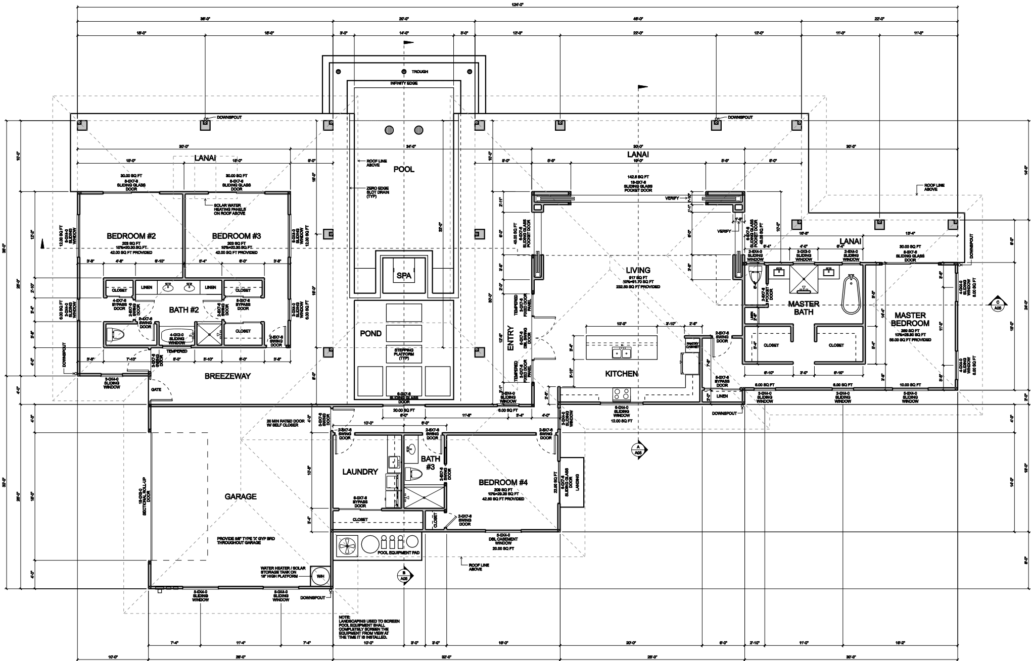
FLOOR PLAN 0' 1" 2" 3" 4" 5" 6" 7" 8" 9" 10" SCALE: 1/4" = 1'-0"
