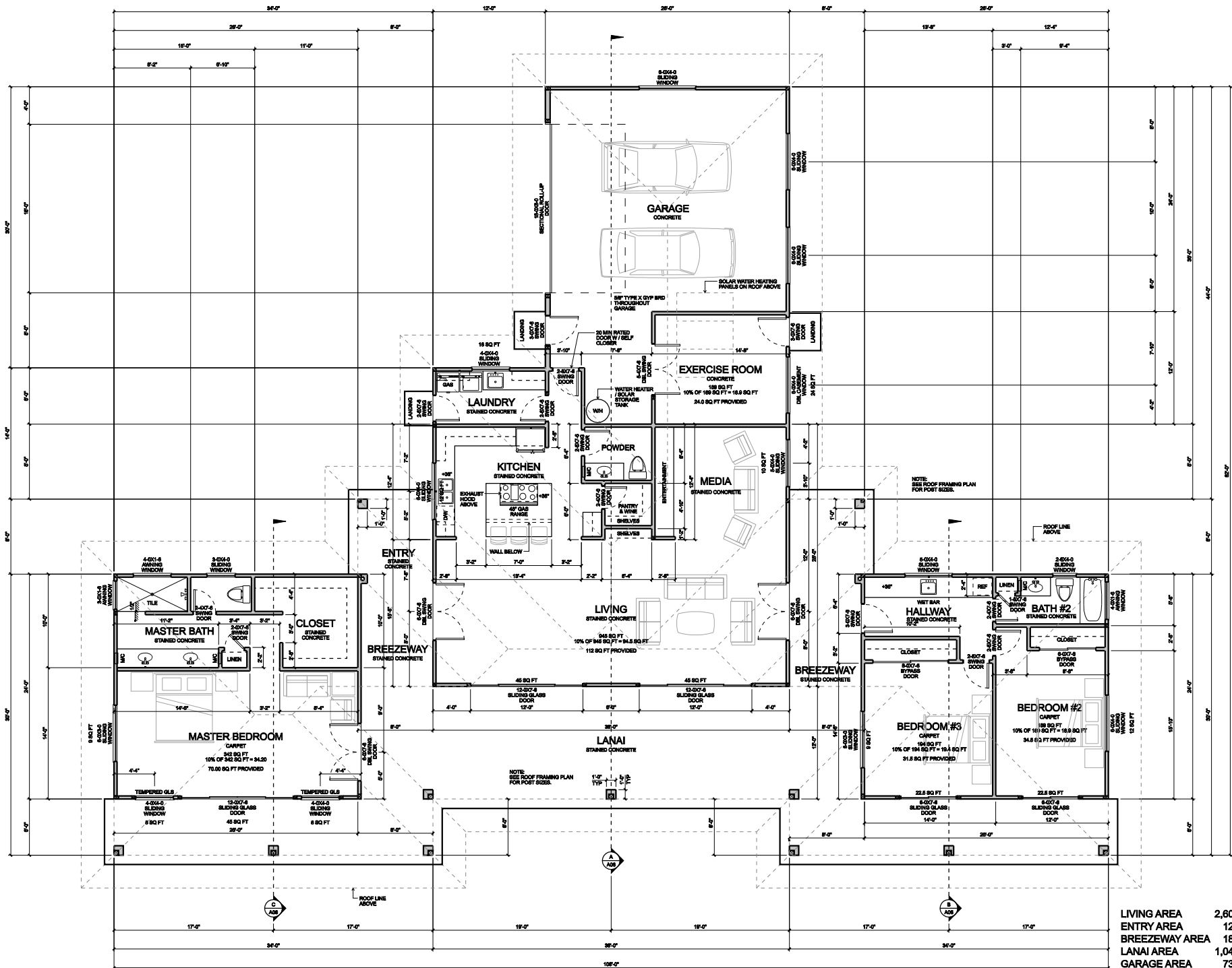
FLOOR PLAN SCALE: 1/4" = 1'-0"
